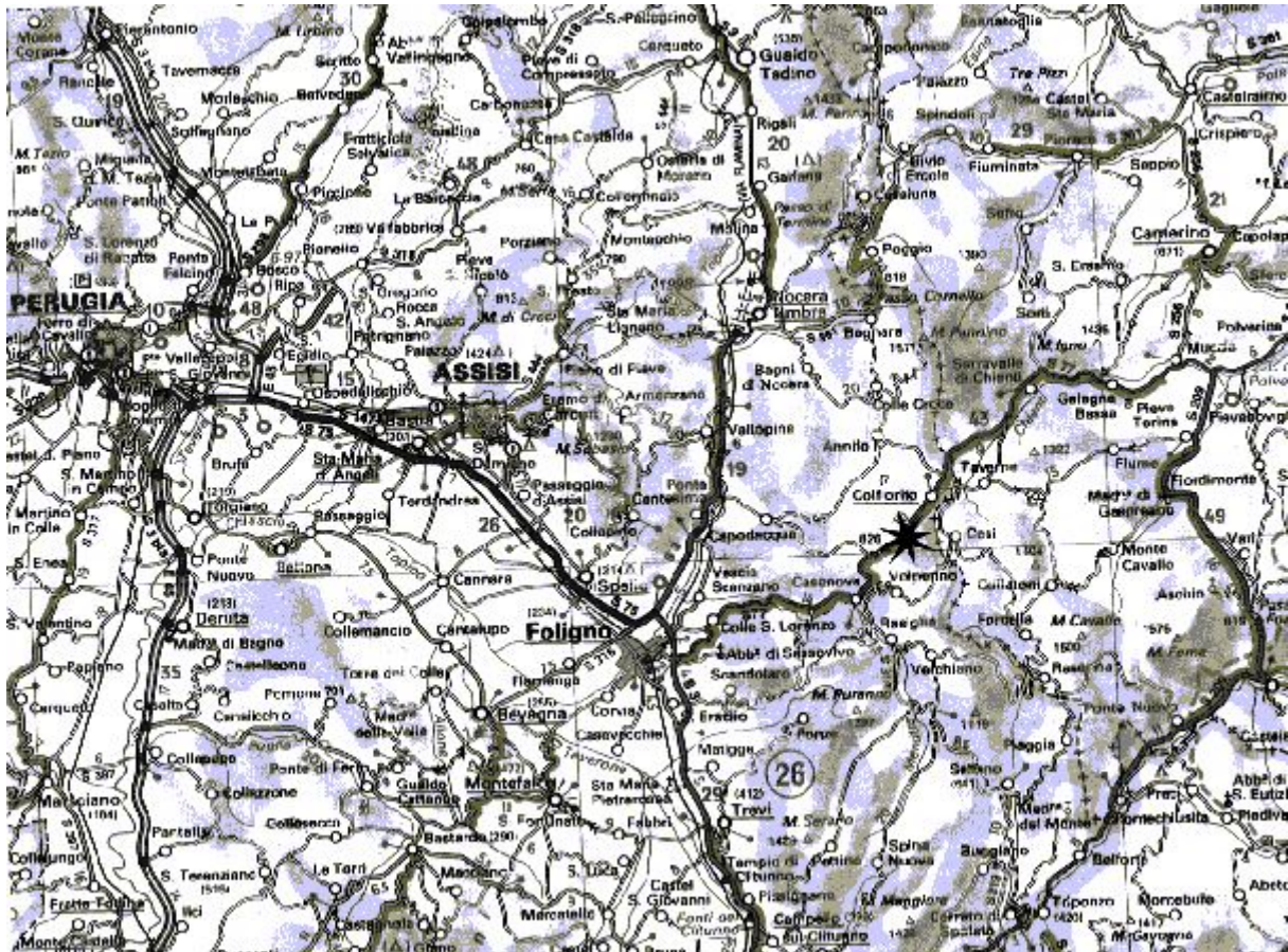
Figure 1: Geographical map of Umbria area in Central Italy showing the earthquake epicenters in Colfiorito and Cesi.
