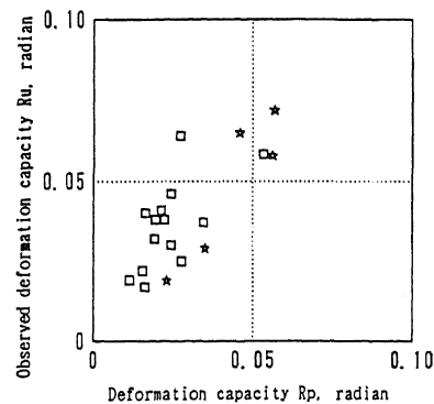
(b) Specimens with deformation capacity derived from potential shear strength (Rf > Rp type)
