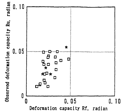
(a) Specimens with deformation capacity derived from flexural analysis (Rf < Rp type)
