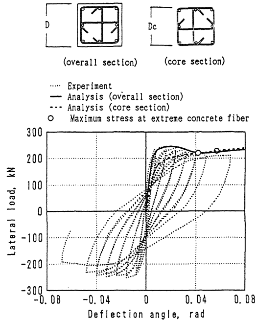
Figure 4. Analytical comparison of load - deflection curves between column with overall section and that with core section only
