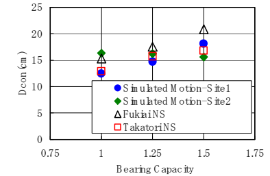
Fig. 25 Vop and Dcon at safety limit of superstructure with different bearing capacities
