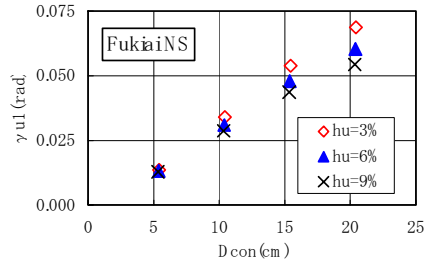
Fig. 22 Effect of damping ratios on story drift angles against observed earthquake motions
