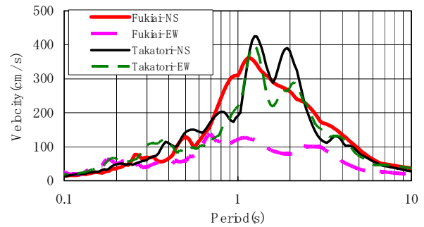
Fig. 17 Pseudo velocity response spectra of earthquake motions at Fukiai and Takatori
