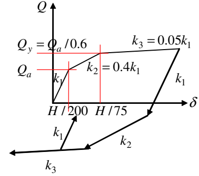
Fig. 15 Relationship between shear force and story drift
