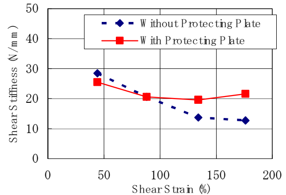
a) Equivalent stiffness
