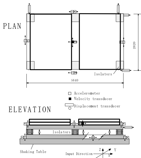
Fig. 1 Outline of seismically isolated model ( \leftrightarrow : parallel to sheet plane)
