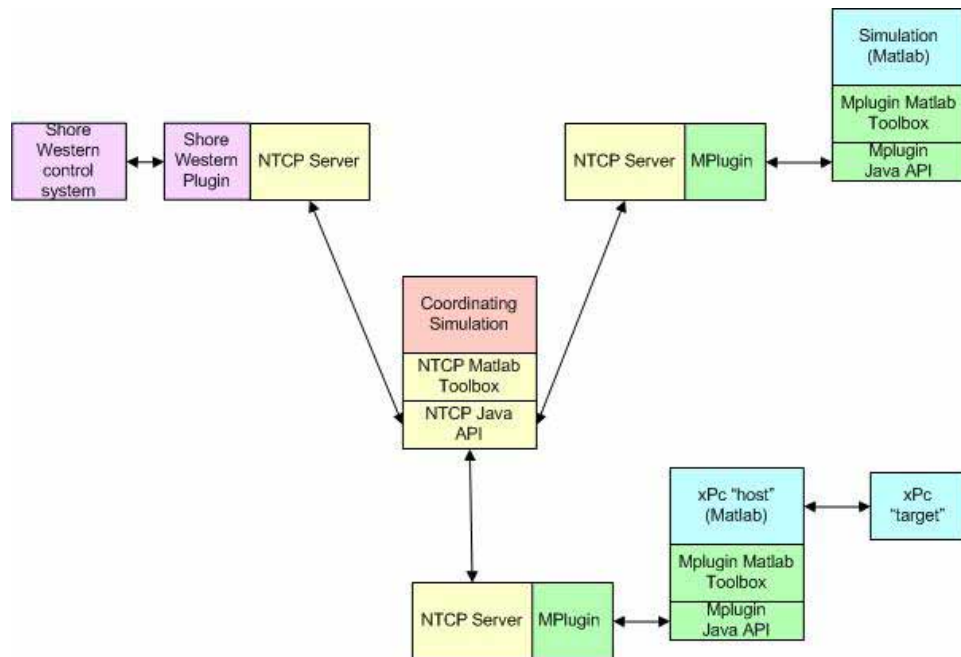
Figure 6: Control Components Used in the MOST Experiment.
