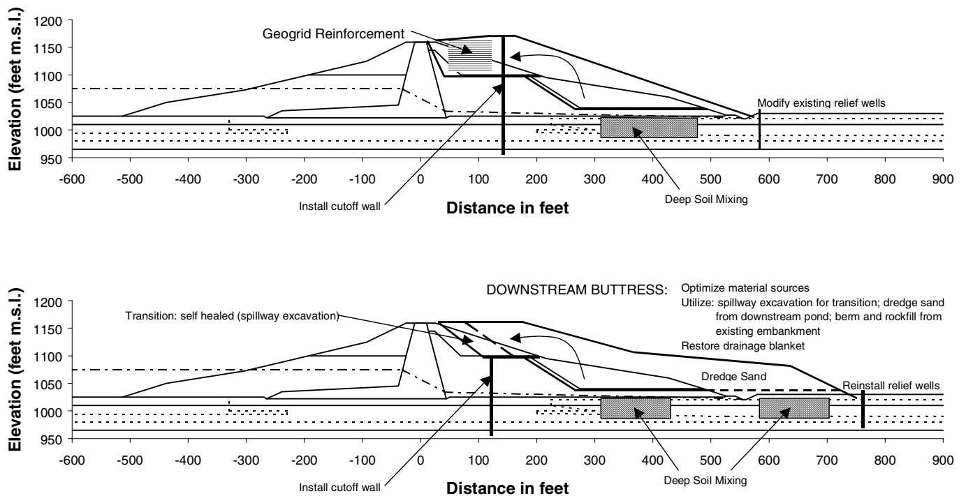
Fig. 8. Preliminary design of the buttress, in two variants
