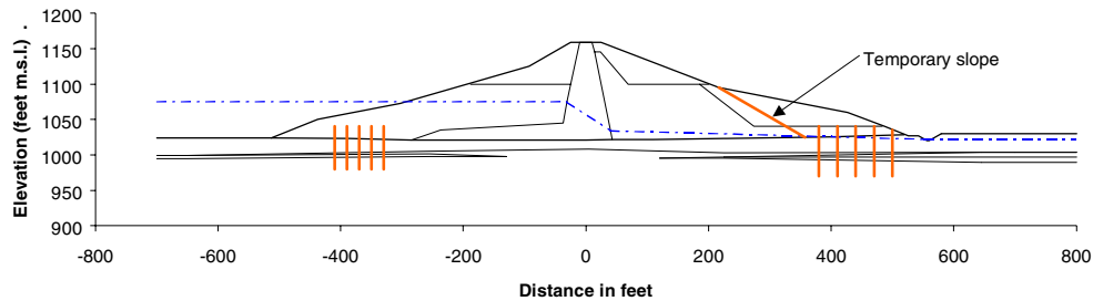
Fig. 4. Reinforcing embankment with piles
