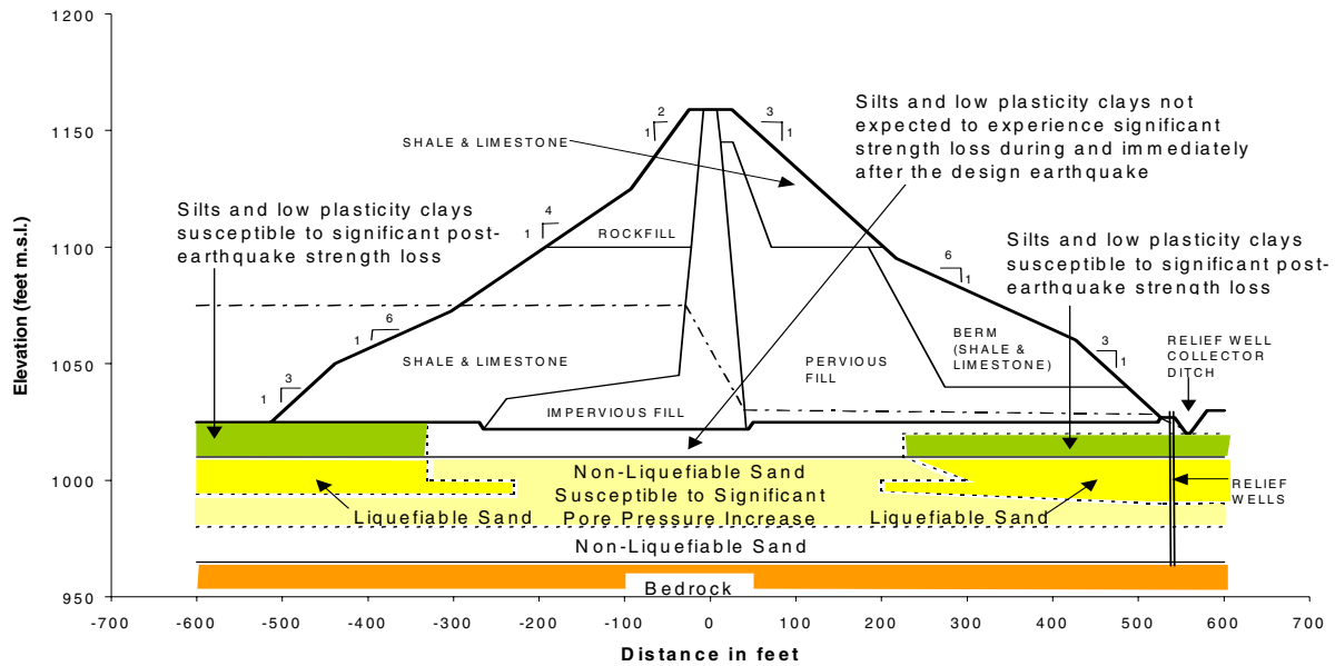
Fig. 1. Cross Section of the Dam (deformed scale).
