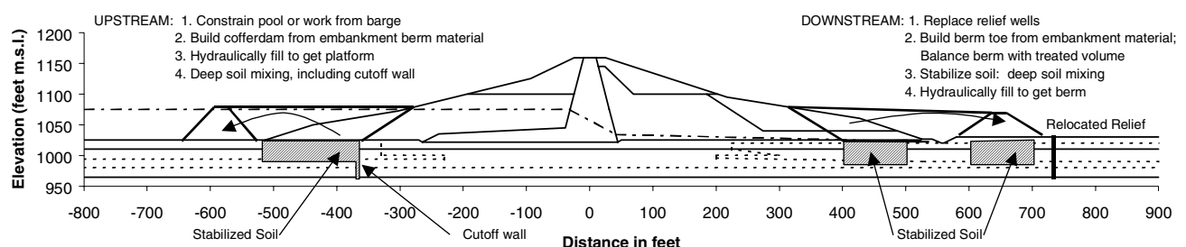
Fig. 7. Berms on stabilized soil, in two variants
