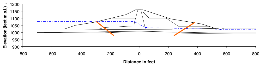
Fig. 5. Reinforcing embankment with anchors
