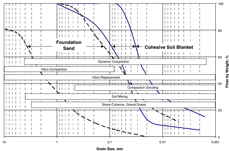
Fig. 2. Foundation soils gradation ranges, vs. ranges of stabilization methods effectiveness (Mitchell [2]).
