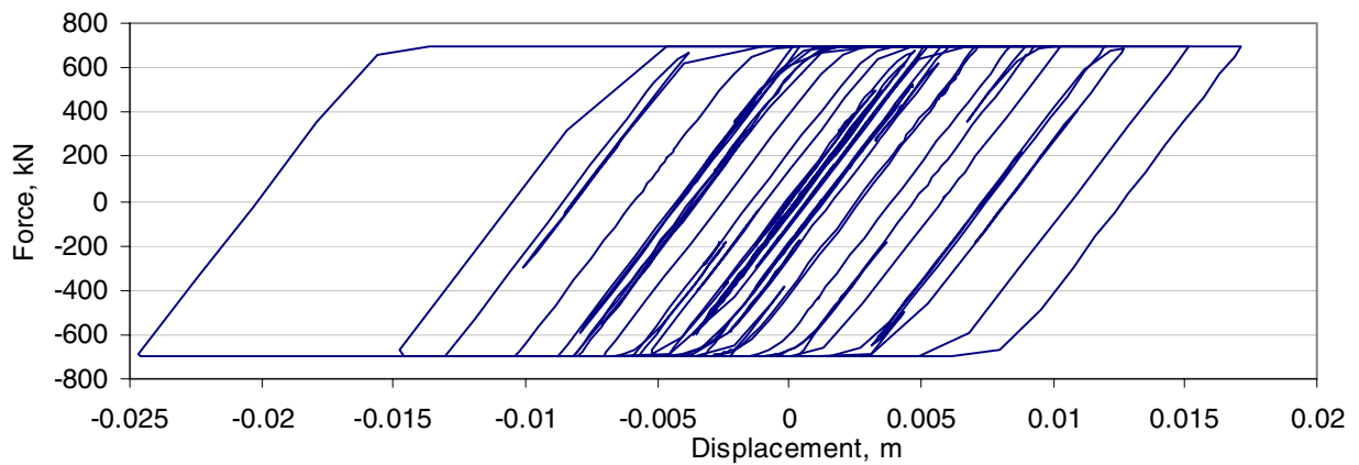
Figure 10. Hysteretic loop of a 700kN friction damper in a diagonal brace
