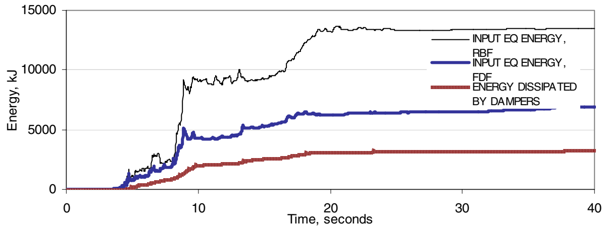
Figure 8. Time histories of energy input and energy dissipated
