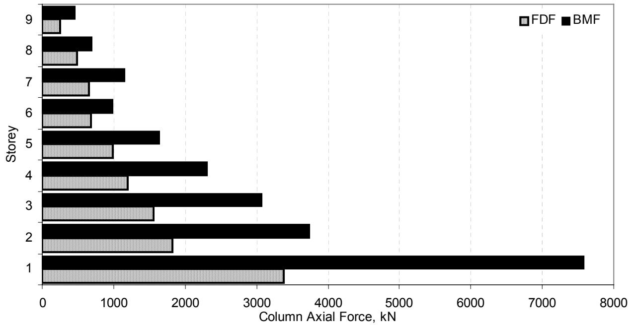
Figure 12. Envelope of column axial force.
