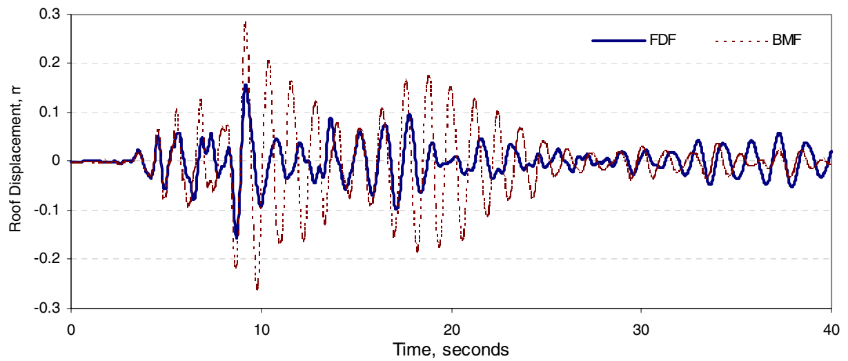
Figure 9. Time histories of displacements at roof
