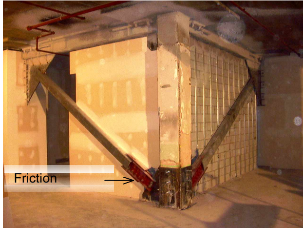
Figure 4. Friction damper in single diagonal brace.
