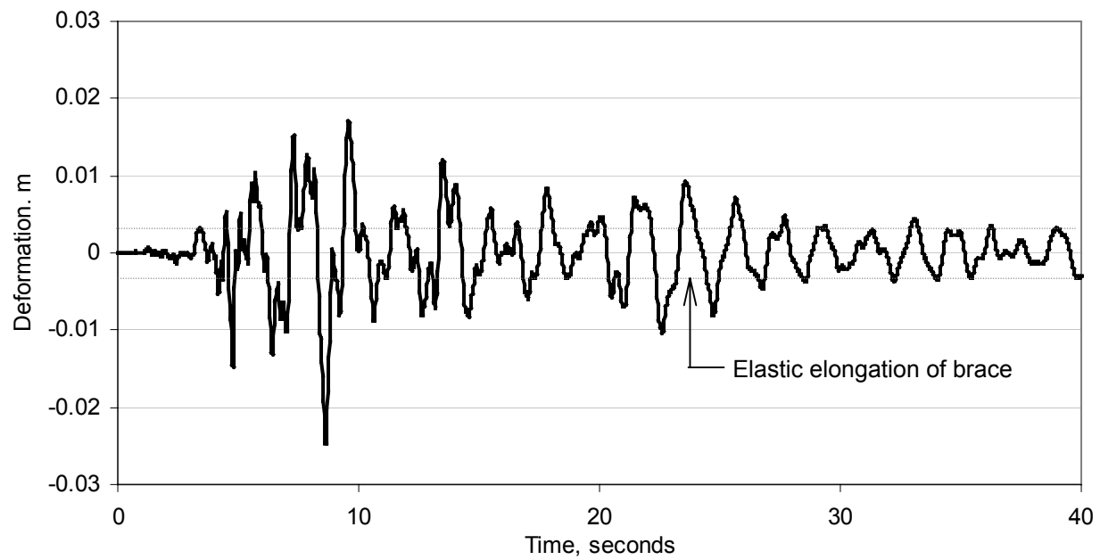
Figure 11. Time history of deformation of damped bracing
