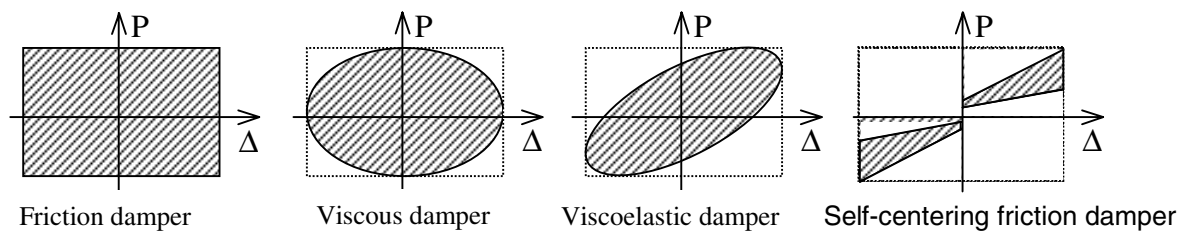
Figure 6. Comparison of hysteresis loops of different dampers
