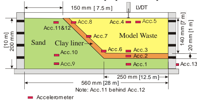
Figure 1 Schematic cross section of the Centrifuge model [prototype dimensions]
