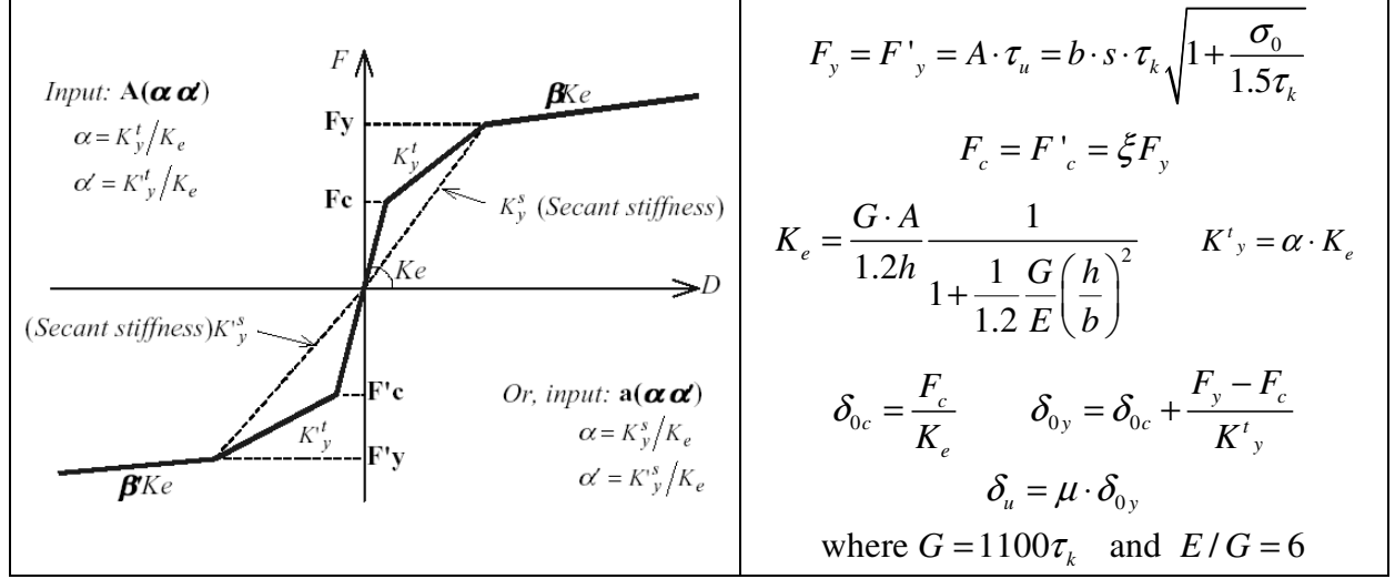
Figure 3. The skeleton curve of masonry panel model and its relevant mechanical characteristics.
