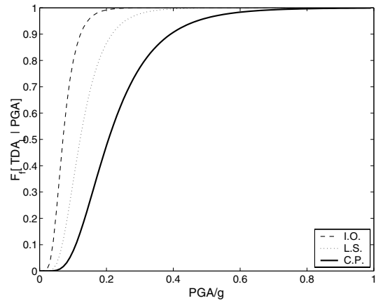
Figure 14. Fragility curves in terms of TDA for the unreinforced panel.
