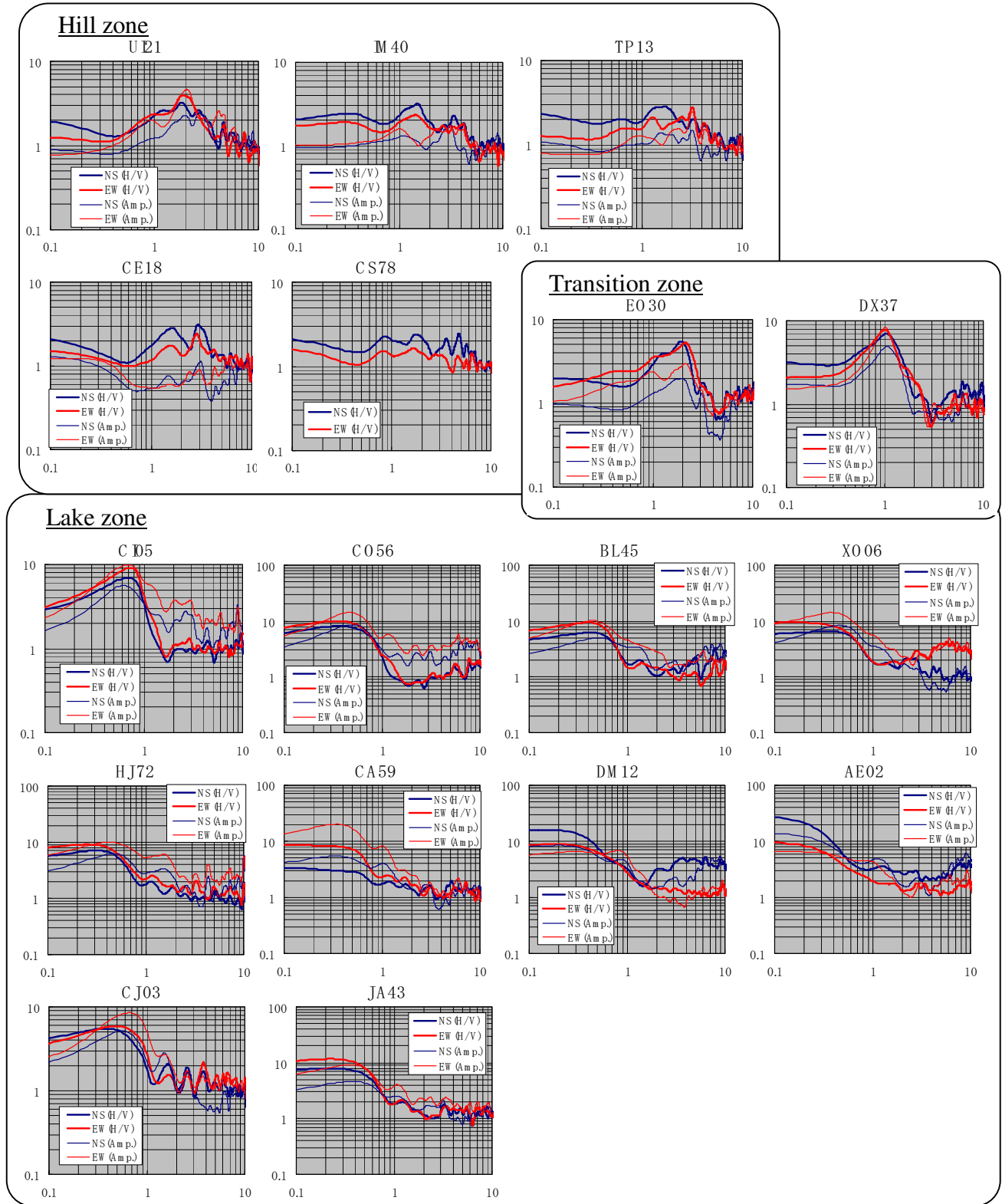
Fig.2 The comparison with the amplification characteristics and the H/V spectral ratio of microtremor on each observation points for strong motion
