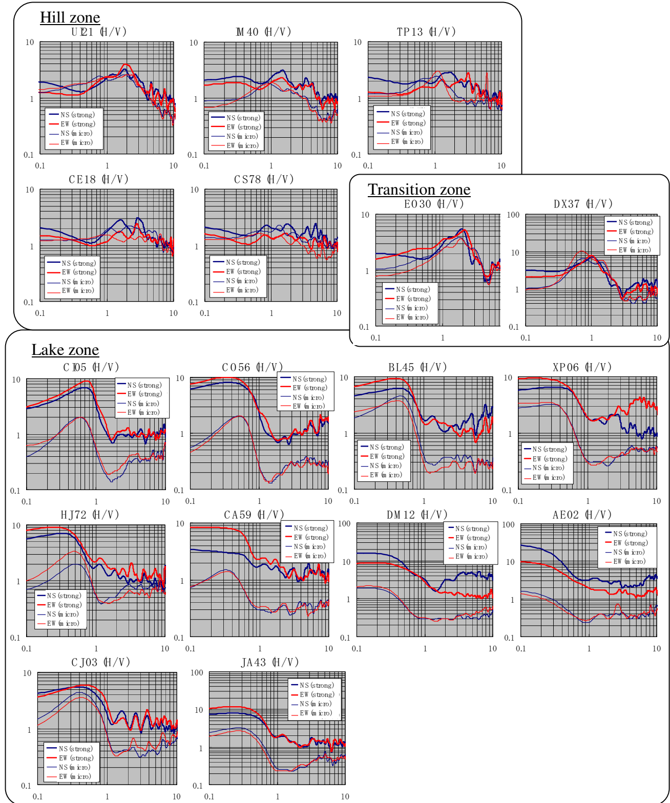
Fig.3 The comparison with the H/V spectral ratio of strong motion and the H/V spectral ratio of microtremor on each observation points for strong motion
