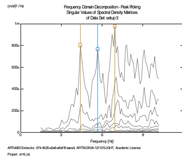
Fig. 18 – House no.16; FDD - station 4
