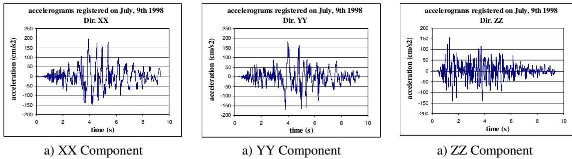
Fig. 2- Accelerograms registered on July, 9th 1998
