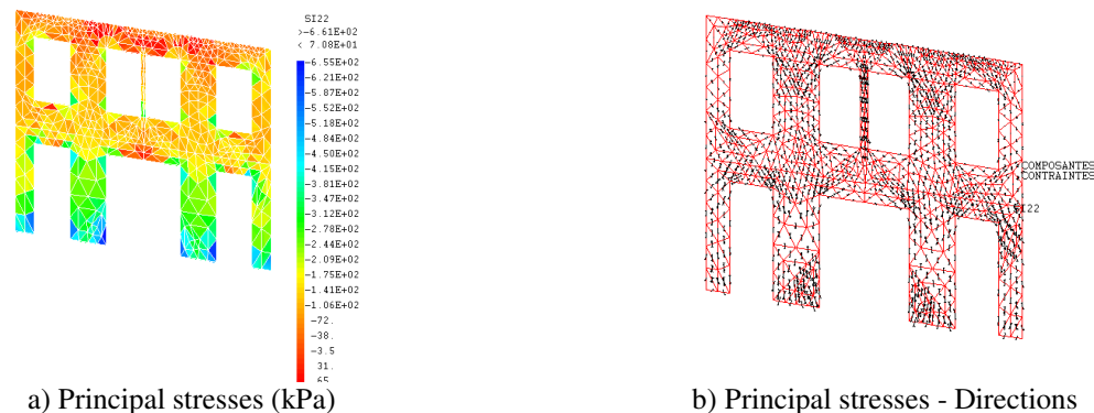
Fig. 25 – House 15 - Principal Stresses (Compression) due to seismic loads – Frontal Wall
