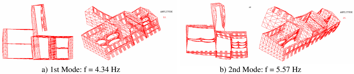
Fig. 22 – House no. 16 – Numerical analysis - Results of modal configurations.
