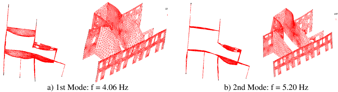
Fig. 20 – House no. 16 – Numerical analysis - Results of modal configurations.
