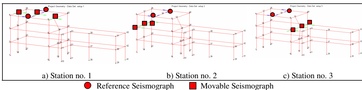
Fig. 16 – House no. 16. Some ambient vibration measuring stations
