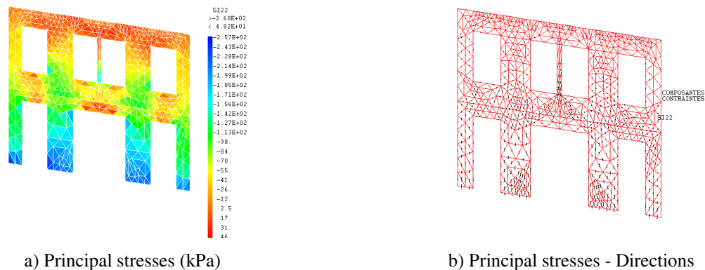
Fig. 23 – House 15 - Principal Stresses (Compression) due to static loads – Frontal Wall
