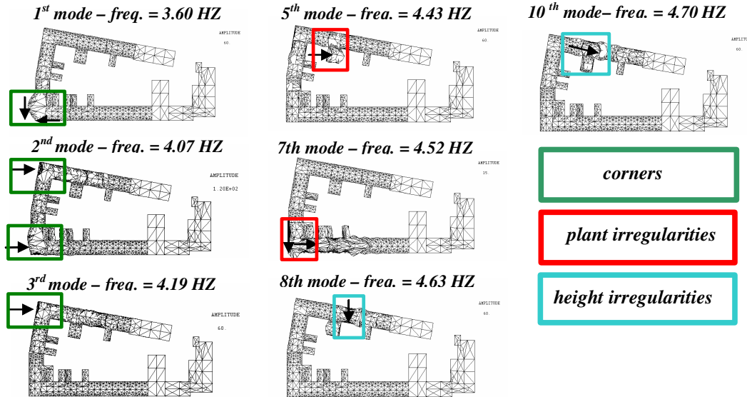
Fig. 11 – Block vibration modes
