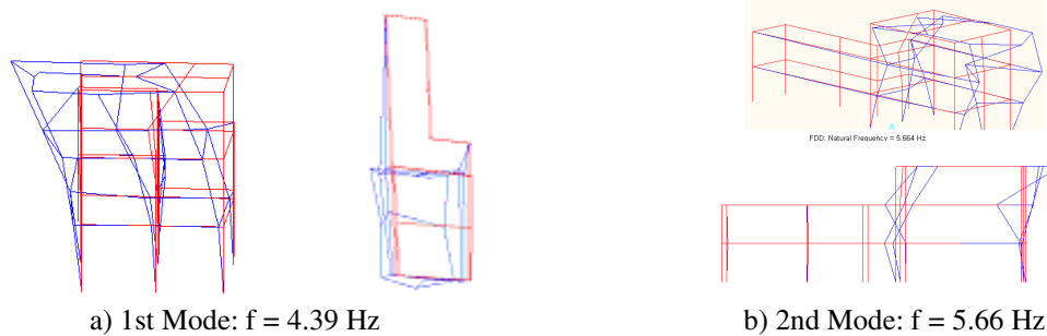
Fig. 21 – House no. 16. Experimental modal analysis – Results of modal configurations.
