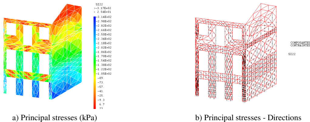
Fig. 24 – House 16 - Principal Stresses (Compression) due to static loads – Frontal Wall
