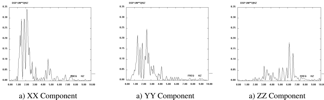
Fig. 3- Power spectra densities of each component during the earthquake on July, 9th 1998.
