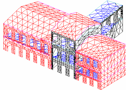
Fig. 14 – House no. 16. Numerical model.
