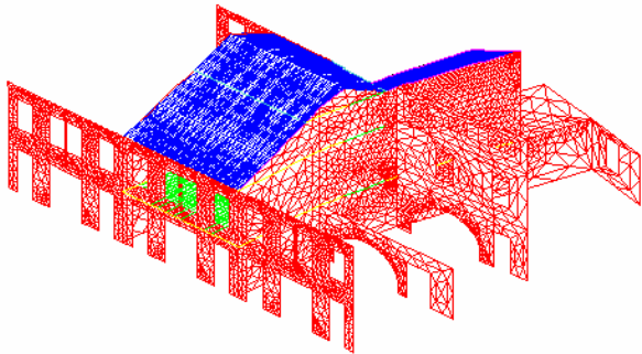
Fig. 13 – House no. 15. New numerical model.
