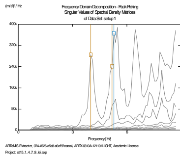
Fig. 17 – House no.15; FDD - station 1
