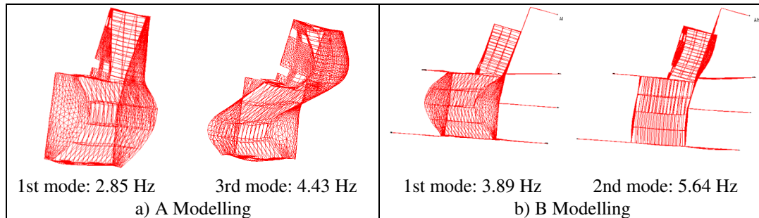
Fig. 7 - Vibration modes of house no. 15. Group effect impact assessment.
