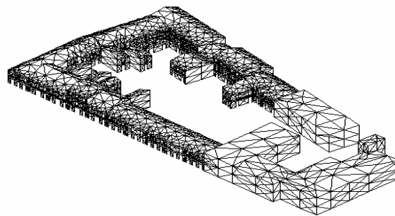
Fig. 10 – Block global modelling
