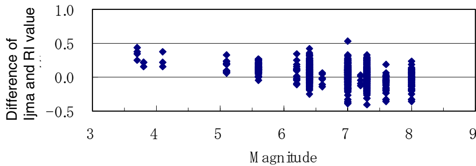
Figure 5 The relationship between magnitude and difference of Ijma and RI value
