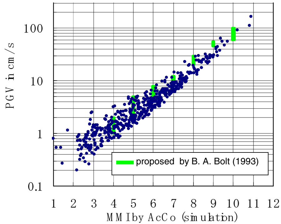
Figure 8 The relationship between instrumental MMI and maximum velocity PGV
