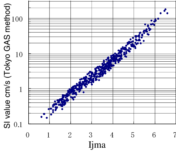
Figure 1 The relationship Ijma and SI value.
