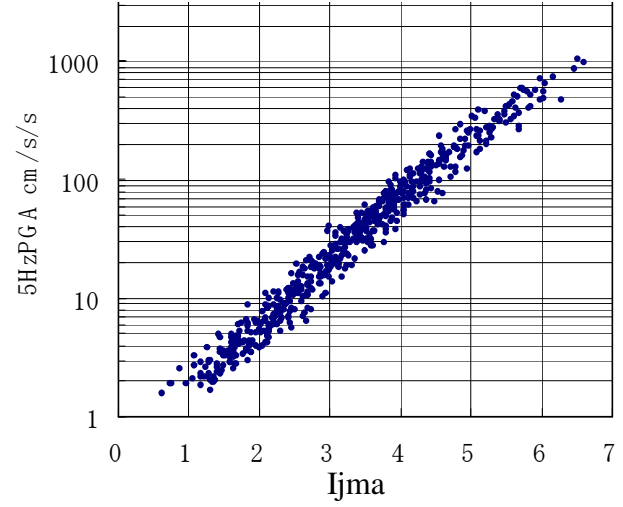
Figure 2 The relationship Ijma and 5HzPGA.
