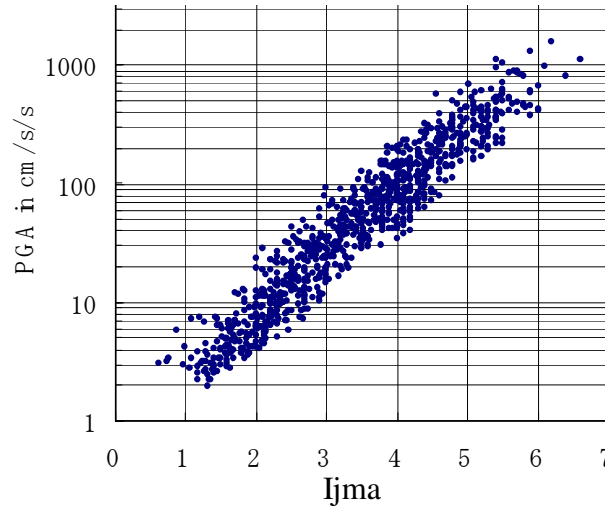
Figure 3 The relationship between Ijma and PGA.
