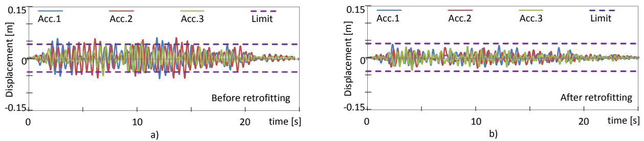
Fig. 8 - Time histories of displacements in transverse direction: a) before retrofitting; b) after retrofitting
