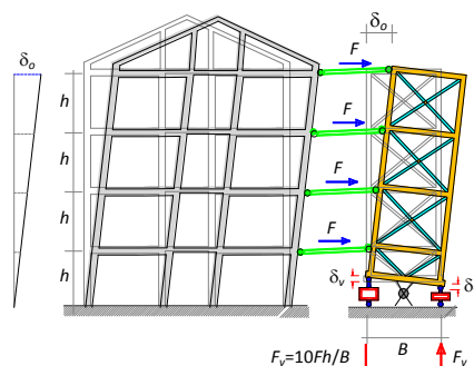
Fig. 2 - System with Dissipative Tower
