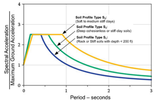
Fig. 2 – Spectral shapes proposed by ATC 3 (1978) for three different soil types codes.
