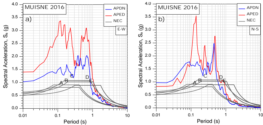
Fig. 11 – Response spectra obtained from Muisne Earthquake, Ecuador
