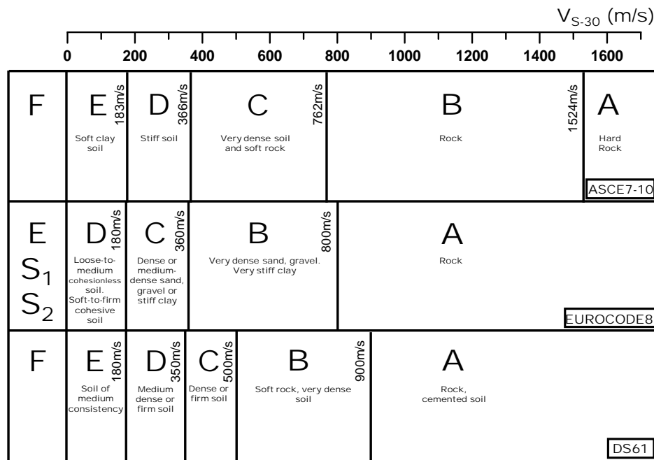
Fig. 3 – Soil classification adopted by ASCE 7, EC-8 and DS61
