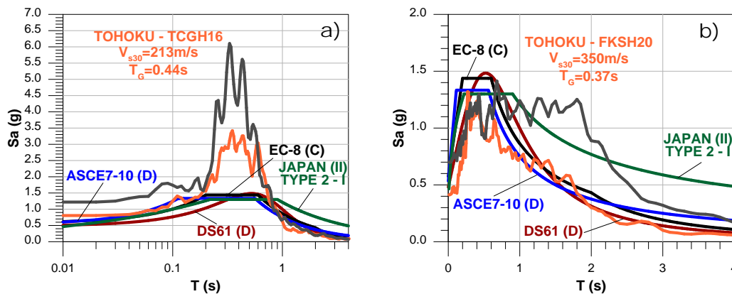
Fig. 10 – Response spectra obtained from records of Tohoku Earthquake. Soil Type II according to JC
