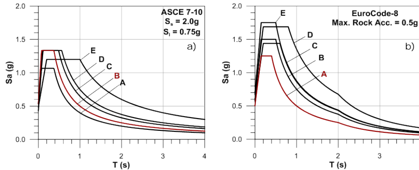
Fig. 4 – Response spectra for the highest respective ground motion. a) ASCE 7 and b) EC-8
