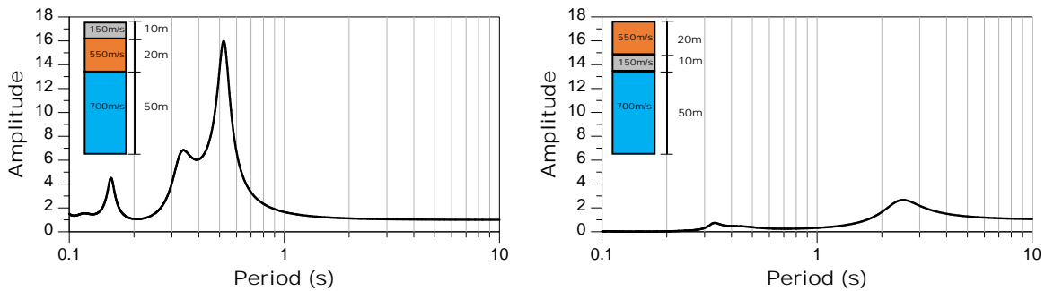
Fig. 12 – Transfer functions of layered grounds
