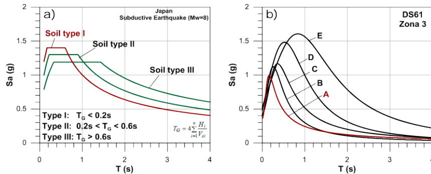
Fig. 5 – Response spectra for the worst subduction ground motion. a) Japanese and b) Chilean codes
