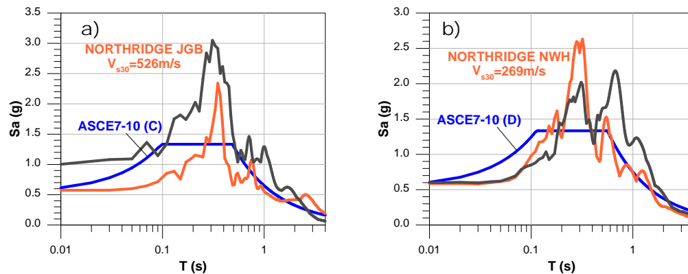
Fig. 9 – Response spectra from records of Northridge Earthquake. Soil Type C - ASCE7
