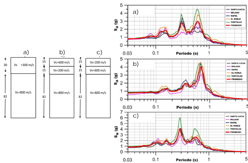
Fig. 13 – Layered soil profiles with same V_{S30} and response spectra at ground surface
