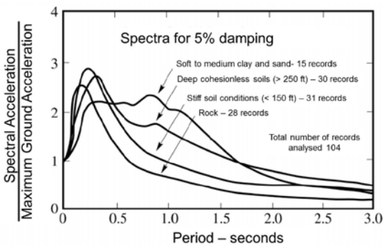
Fig. 1 – Average acceleration spectra for different site conditions (Seed et al. 1976)
