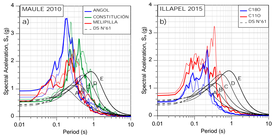
Fig. 7 – Response spectra obtained from Chilean Earthquakes a) Maule and b) Illapel
