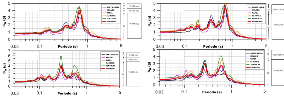
Fig. 14 – Response spectra of layered ground (left) and using V_{S30-E} (right)
