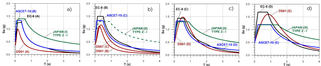
Fig. 6 – Response spectra according to soil conditions in different codes.
