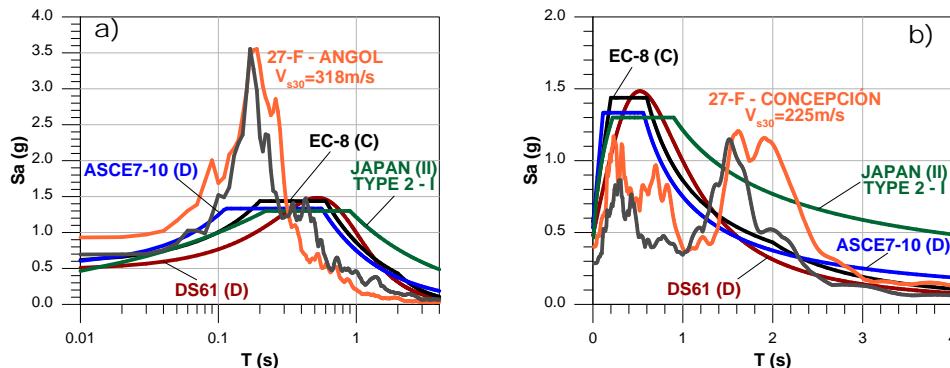
Fig. 8 – Response spectra obtained from records of Maule Earthquake. Soil Type D according to DS61
