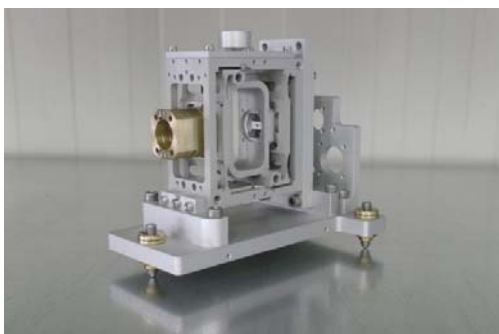
Fig. 4 – Uniaxial monolithic Unisa Folded Pendulum (Model GE15).
