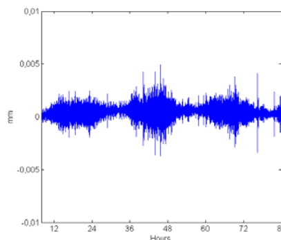
Fig. 9 – Displacement time course of the lateral transverse measurement point on the top of Trajan Arch (II test).
