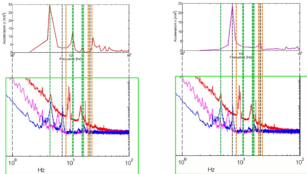
Fig. 14 15 – Amplification function comparison for longitudinal and transversal direction-central node
