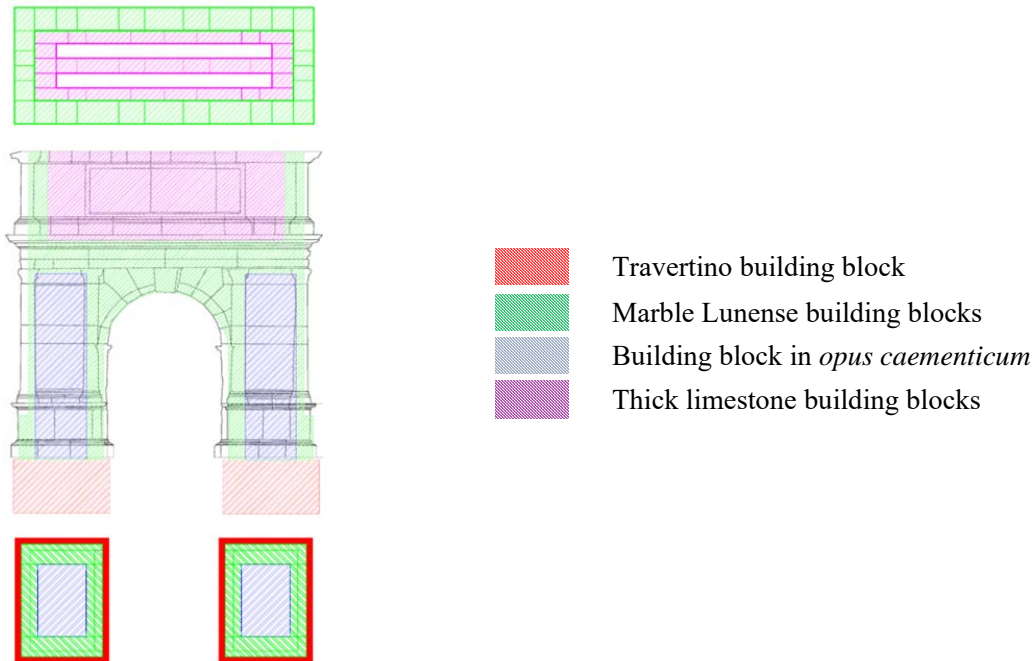
Fig. 10 – Macro-elements subdivision of the Arch, with breakdown by material.
