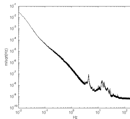
Fig. 8 – Displacement spectral density of the central transverse measurement point on the top of Trajan Arch (II test).
