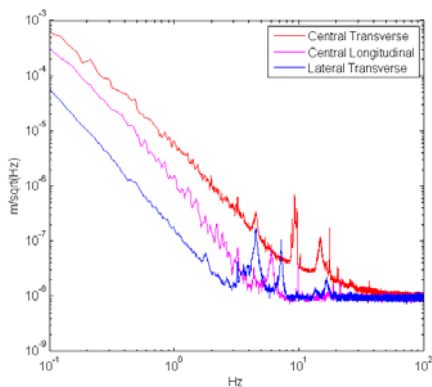
Fig. 7 – Displacement spectral density of selected measurement points on the top of Trajan Arch (I test).
