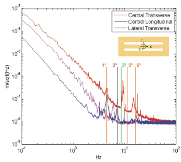
Fig. 13 – Comparison between numerical and signals data analyses. Reference Case 2
