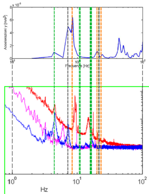
Fig.16 – Amplification function comparison for lateral transverse direction-corner node
