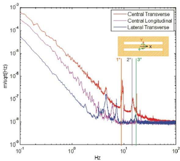
Fig. 12 – Comparison between numerical and signals data analyses. Case 1
