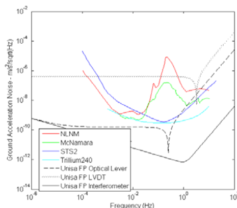
Fig. 6 – Sensitivity curves of the Unisa Horizontal Folded Pendulum mechanical sensors equipped with an Optical Lever, a LVDT and a Michelson Interferometer readouts and tuned at different resonance frequencies, compared with the Peterson Low Noise Model, with the McNamara Noise Model and with two commercial sensors: STS-2 by Streckeisen and Trillium-240 by Nanometrics.
