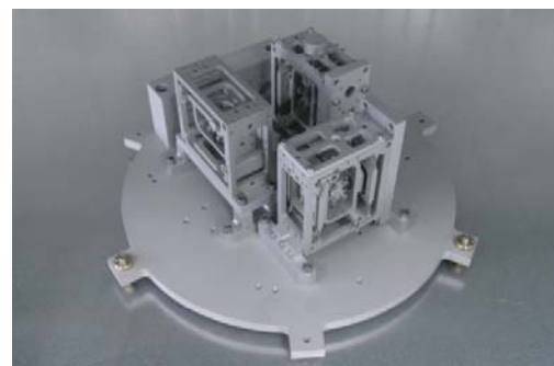
Fig. 5 – Triaxial sensor based on monolithic Unisa Folded Pendulum.
