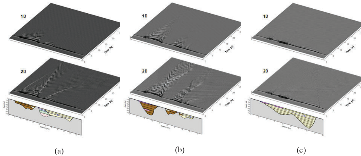
Fig. 3 – Transverse component of motion at the surface of the (a) NS, (b) EW, and (c) CD cross-sections for an incident SH-wave. Upper panels are the results of 1 D models (M4) and lower panels are those of the 2D models (M2).
