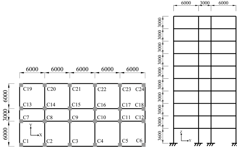
Fig. 1 – Plan view (left) and elevation view (right) of the ten-story rc building adopted for the current study.
