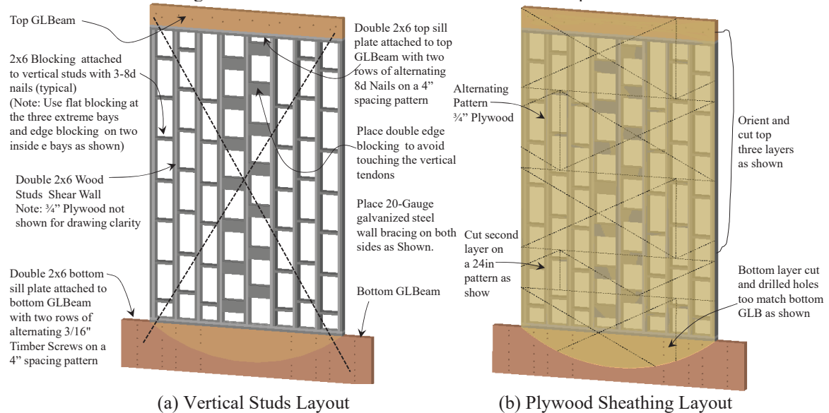
Fig. 2 – X-Braced Wood Panel Shear Wall Sheathed with Wood Structural Panels
