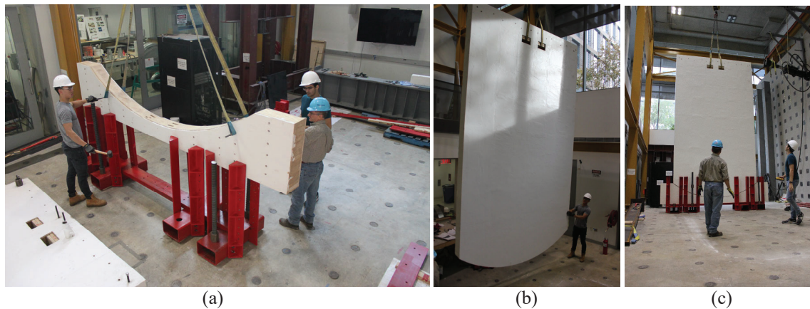
Fig. 3 – Wall Construction and Installation of Top and Bottom Glulam Beams
