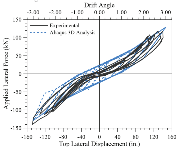
Fig. 10 – In-Plane Load Deformation Response
