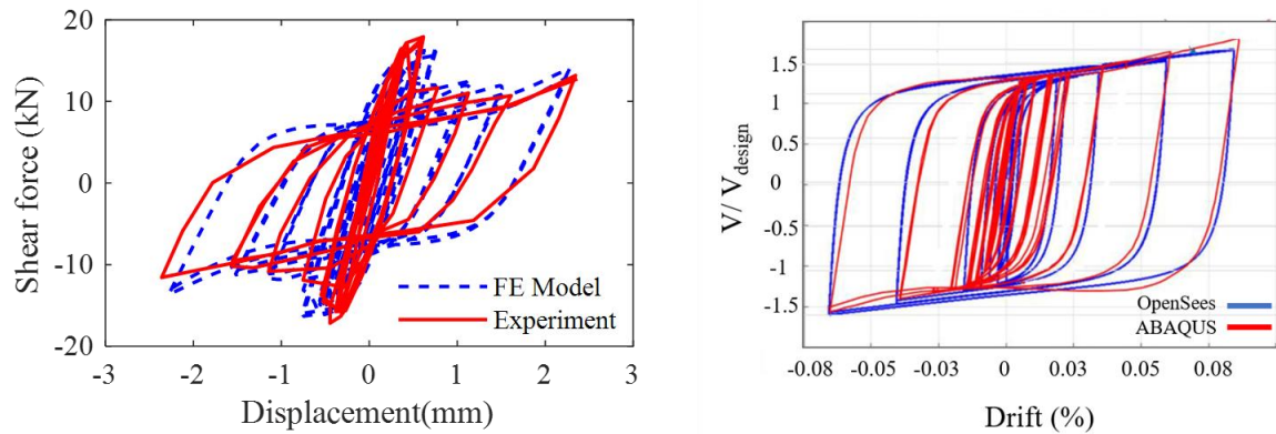
Fig 4 – Verification of the modeling approach: (a) comparison of ABAQUS and experimental results (b) OpenSees and ABAQUS model
