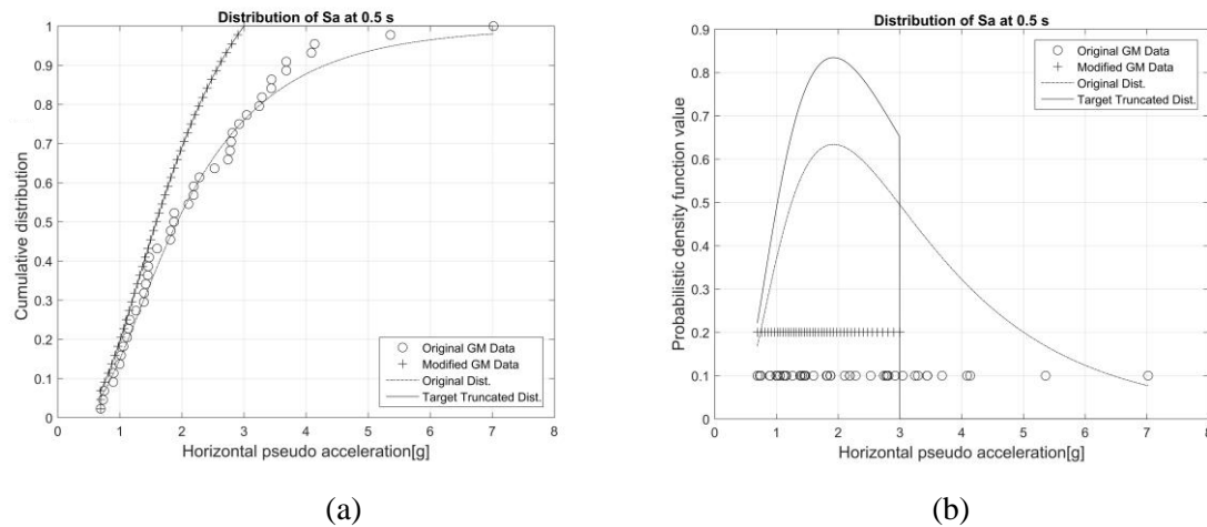
Fig. 2 –Distribution of the ground motion value. (a) Cumulative distribution (b) Density function value
