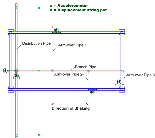
Fig. 9 – Instrumentation for responses discussed herein
