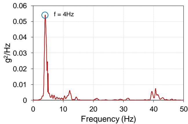
Fig. 8 – Power spectrum of distribution pipe acceleration
