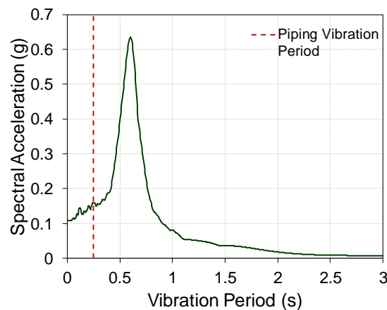
Fig. 7 – Response spectrum of input motion
