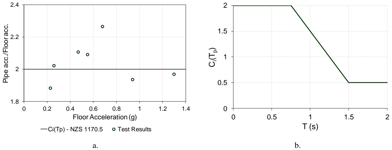
Fig. 10 – a) Distribution pipe acceleration amplification; b) Spectral shape coefficient [7]
