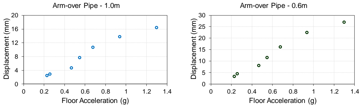
Fig. 11b – Displacement demands on different segments of piping
