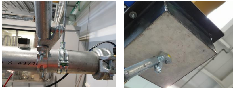
Fig. 6 – Brace and hanger rod attachments
