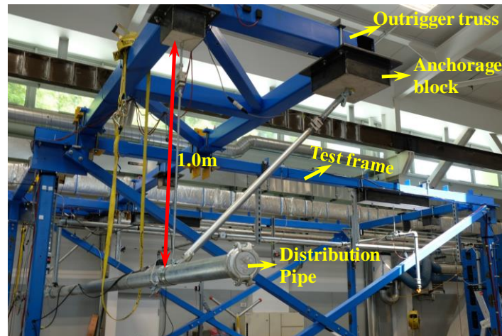
Fig. 3 – Different components of the test setup
