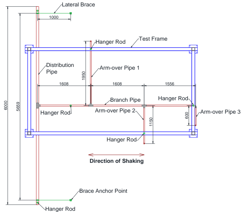
Fig. 5 – Test setup plan view
