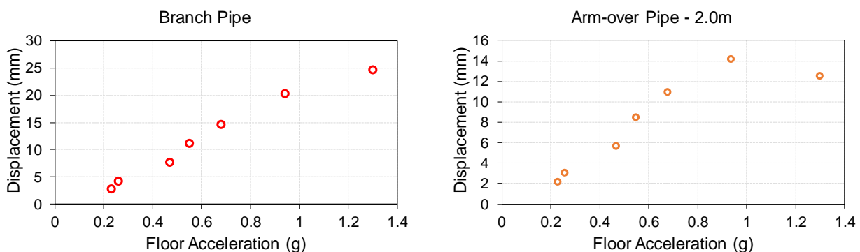
Fig. 11a – Displacement demands on different segments of piping
