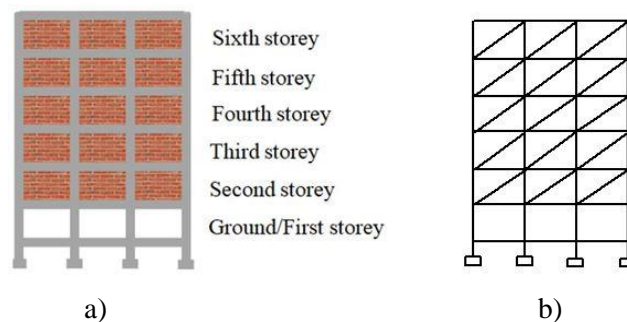
Fig. 1 a) Open Ground Storey b) Equivalent SAP model in 2D
