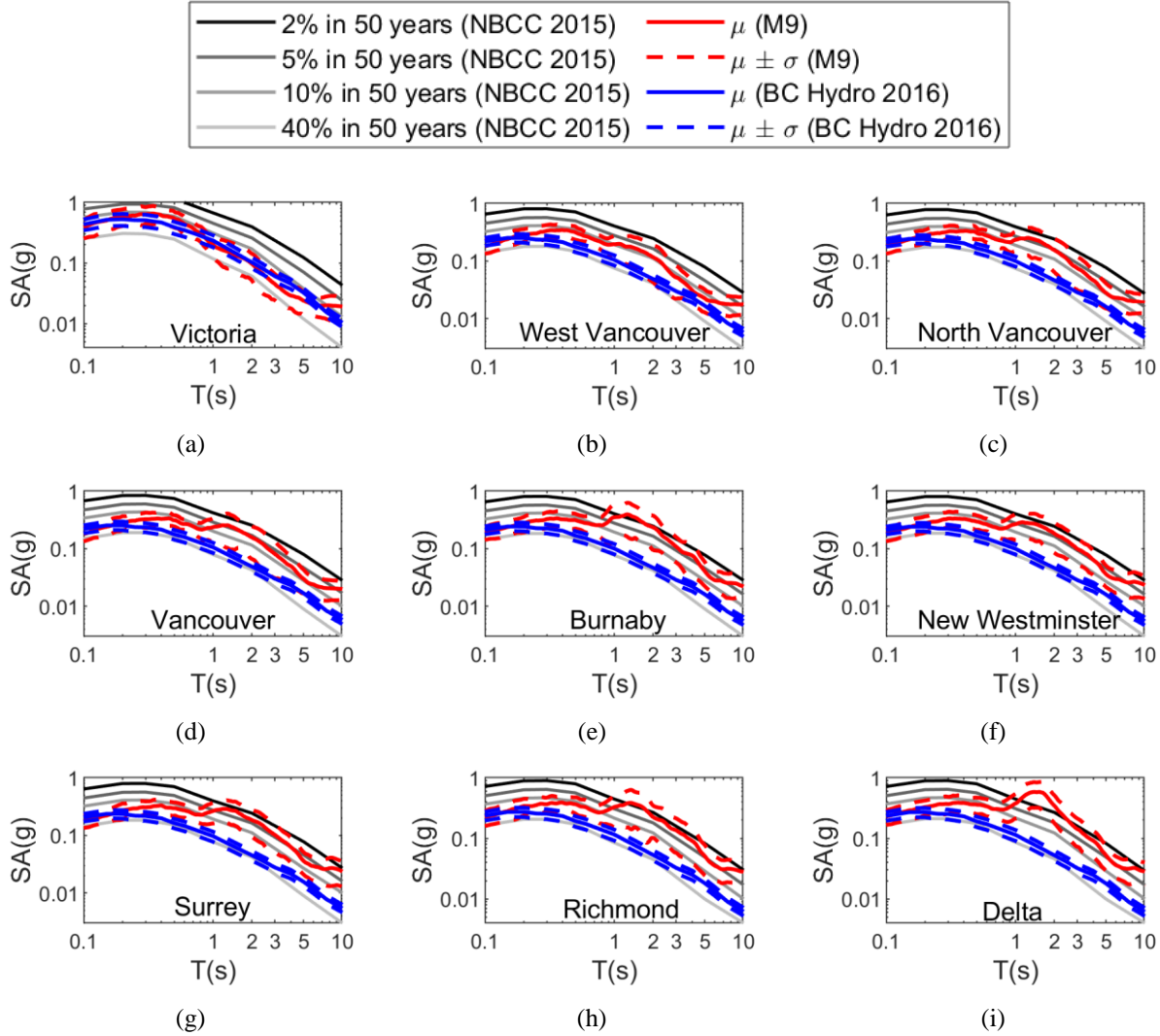
Fig. 2. Average response spectra of simulated M9 CSZ earthquake ground motions, BC Hydro estimates and NBCC 2015 probabilistic estimates of the hazard with 2%, 5% 10% and 40% probability of exceedance in 50 years in (a) Victoria, (b) West Vancouver, (c) North Vancouver, (d) Vancouver (e) Burnaby, (f) New Westminster, (g) Surrey, (h) Richmond and (i) Delta. Adapted from [25].
