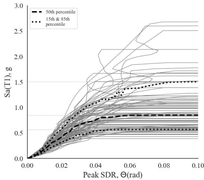
Fig. 8– Incremental dynamic analysis (IDA) curves
