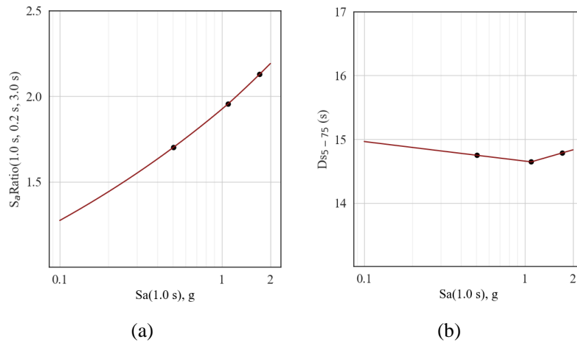
Fig. 2 – Median (a) S_a Ratio(1.0 s, 0.2 s, 3.0 s) and (b) D_{S5-75} targets, conditional on different levels of S_a(1.0 \text{ s}) .
