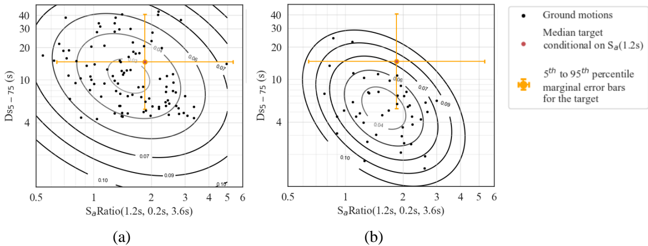
Fig. 10 – Contour plots of the standard error in predicting the median collapse intensity, overlaid on the S_a Ratio and D_{55-75} values of the (a) selected record set and (b) the FEMA P695 far field set, and the 5 th to 95 th percentile marginal error bars of the S_a Ratio and D_{55-75} targets conditional on the 2% in 50 year exceedance probability of S_a(1.2s) .
