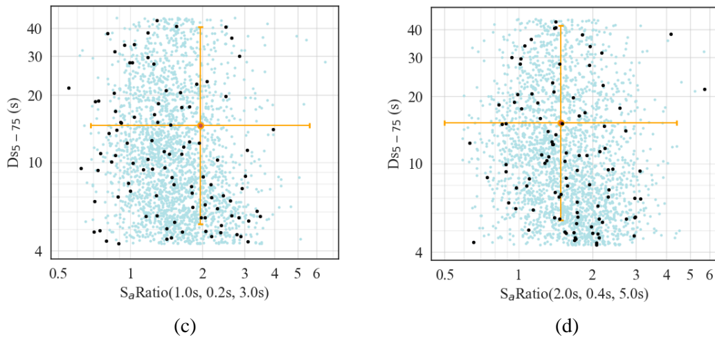
Fig. 6 – S_a Ratio and D_{S5-75} values of the selected and candidate ground motions overlaid on the targets conditional on the 2% in 50 year exceedance probability of S_a at (a) 0.2 s, (b) 0.5 s, (c) 1.0 s, and (d) 2.0 s
