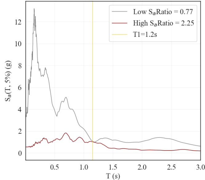
Fig. 1 – Response spectra of two ground motions scaled to a common value of S_a(1.2s) = 1g with low and high S_a \text{Ratio}(1.2s, 0.2s, 3.6s) values.
