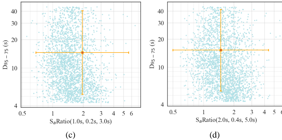
Fig. 3 – Candidate ground motions and the distributions of the S_a Ratio and D_{S5-75} targets conditional on the 2% exceedance probability of S_a at (a) 0.2 s, (b) 0.5 s, (c) 1.0 s, and (d) 2.0 s
