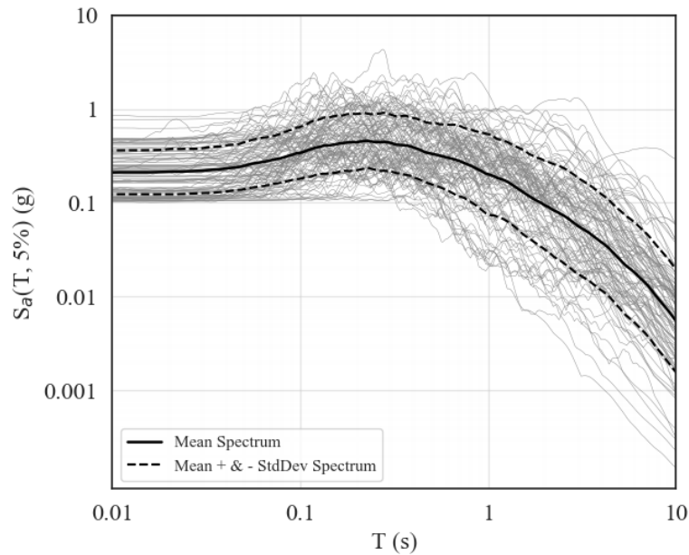
Fig. 5 – Response spectra of the 100 selected records.
