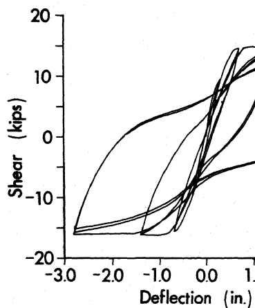
Figure 10. Specimen 3, 6mm spiral.
