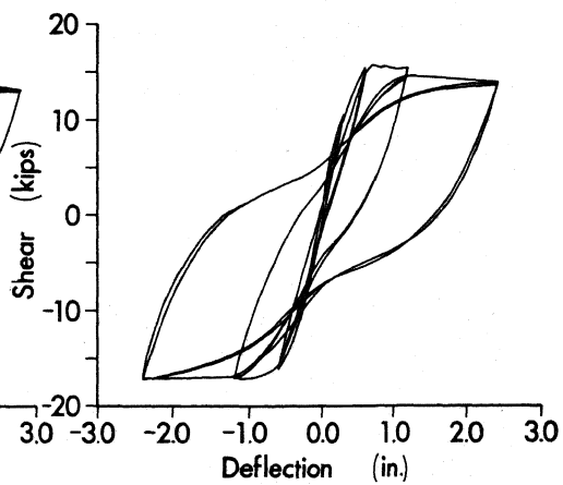
Figure 11. Specimen 4, U-clamps.
