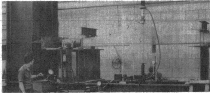
Figure 2. Specimen 1 in test frame.
