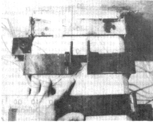
Figure 7. Specimen 4, U-clamps; cracking at maximum deflection.
