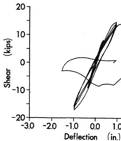
Figure 8. Specimen 1, unstrengthened.
