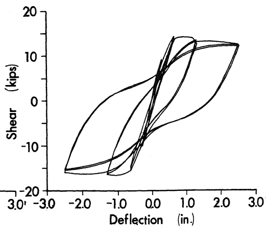
Figure 9. Specimen 2, bands.
