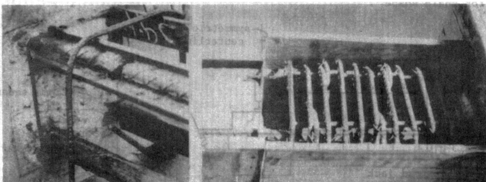
Figure 4. Repair for Specimen 1R: #7 bar welded to 50 mm angles (left), 9.5 mm hoops at 38 mm spacing (right).
