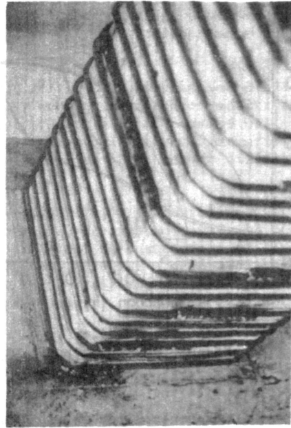
Figure 6. Specimen 3, 6 mm rectangular spiral.
