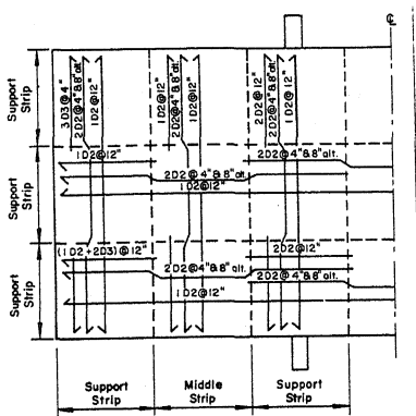
Fig. 2 Reinforcement Details
