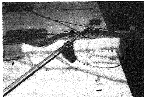
Fig. 6 Crack Pattern of Panel 2 Specimen F-1
