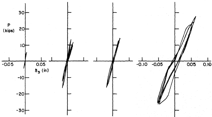
Fig. 8 Hysteresis Diagrams of Panel 2, Specimen F-1
