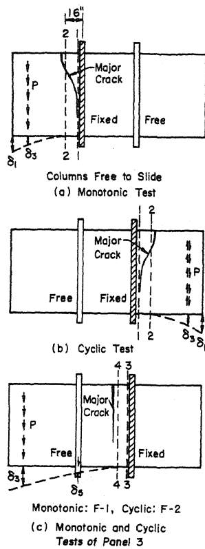
Fig. 5 Ultimate Strength Tests
