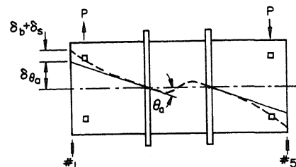
(b) Anti-symmetrical Loading
