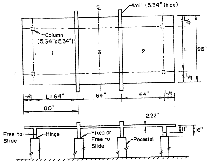
Fig. 1 Test Specimen and Support Conditions
