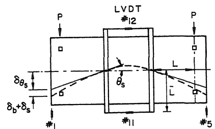
(a) Symmetrical Loading
