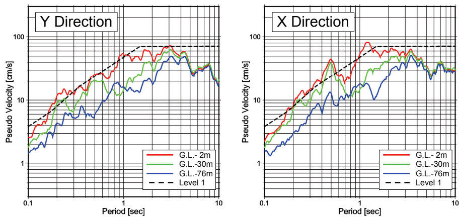
Figure 6. Pseudo velocity response spectra ( h=5\% ) of ground motion recorded at Shinkiba site during the Great East Japan earthquake. The standard pseudo velocity spectra of Level 1 ground motion of Specifications for Highway Bridges (Japan Road Association 2002) is indicated in a broken line.
