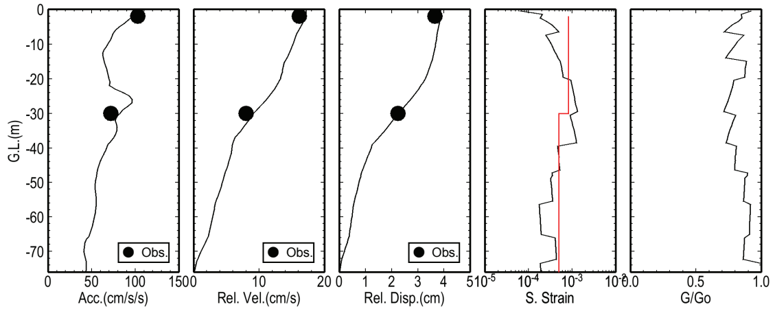
Figure 9 Depth distribution of maximum response calculated by earthquake response analysis. A filled circle and red line had indicated observation results. Red line into the shear strain distribution is averaged shear strain calculated from observation record.
