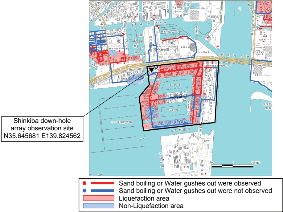
Figure 4. Liquefaction investigation results around Shinkiba down-hole array observation site after the 2011 off pacific of Tohoku earthquake (Revised MLIT and JGS 2011).
