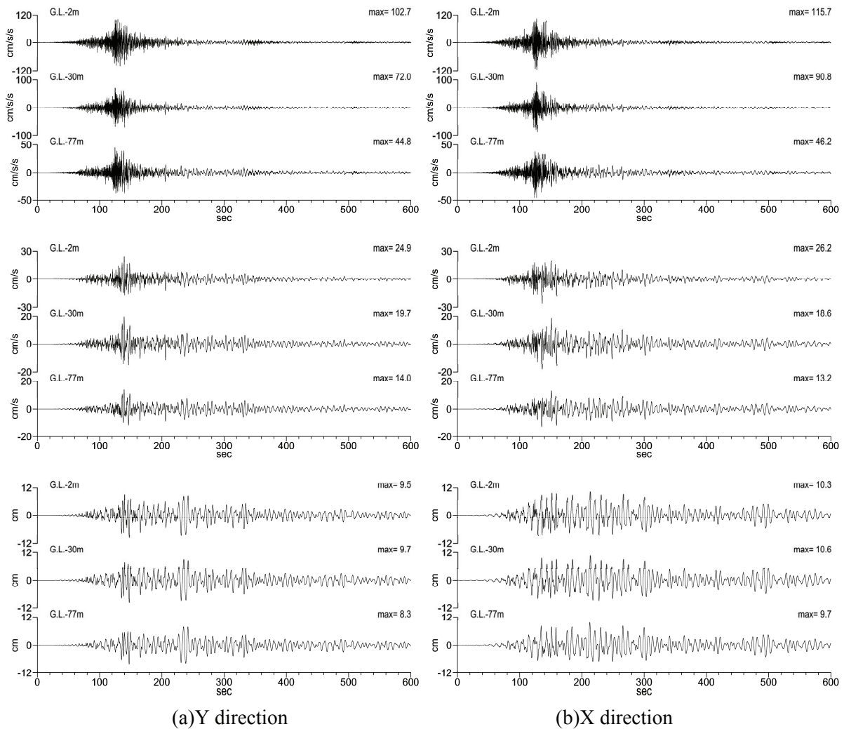
Figure 5. Waveform of observation record at Shinkiba site from main event.
