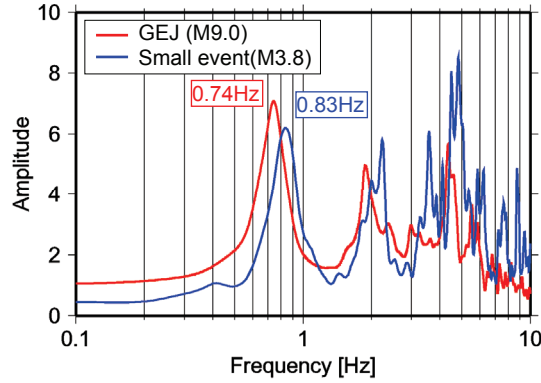
Figure 7. Comparison between the Great East Japan earthquake (M9.0) and small event(M3.8) transfer function
