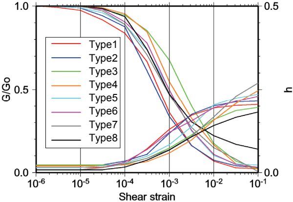
Figure 8. Nonlinear properties which are G/Go - \gamma and h - \gamma of each layers
