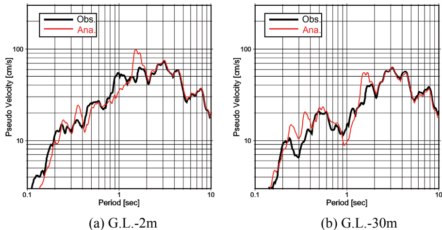
Figure 11. Comparison of the pseudo velocity response spectra (PVRs) with damping factor of 0.05 of the analyzed motion and observed motion at G.L.-2m and G.L.-30m. A black line means observation and a red line means analysis.
