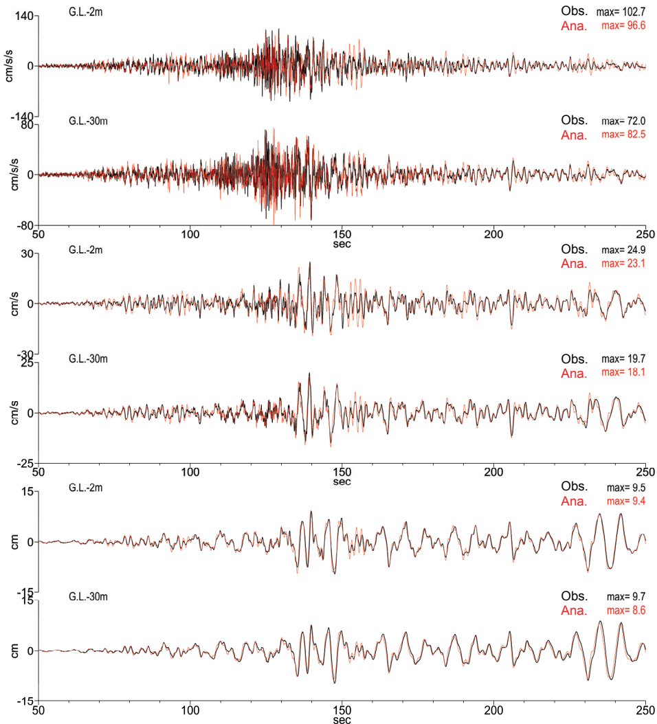
Figure 10. Comparison of an observation waveform and an analysis waveform at G.L.-2m and G.L.-30m. A black line means observation and a red line means analysis.
