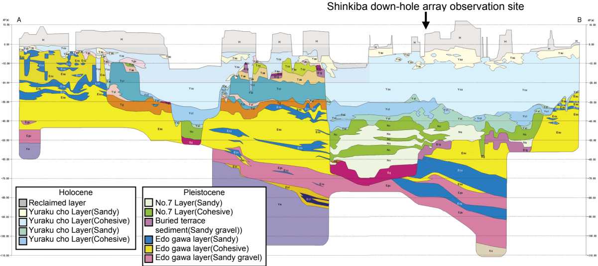
Figure 3. Geological cross-section around downhole array observation site.
